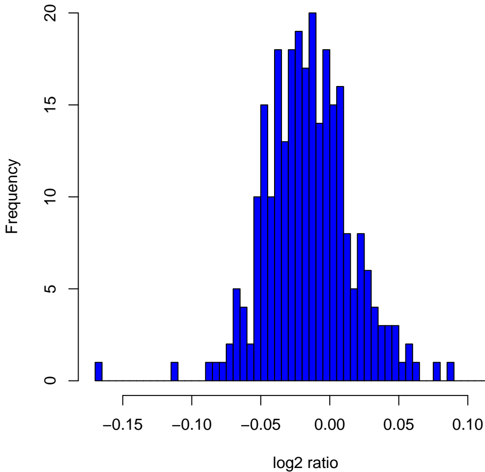
Histogram of log 2 ratios in 270 HapMap samples at clone Chr1tp-3G11
