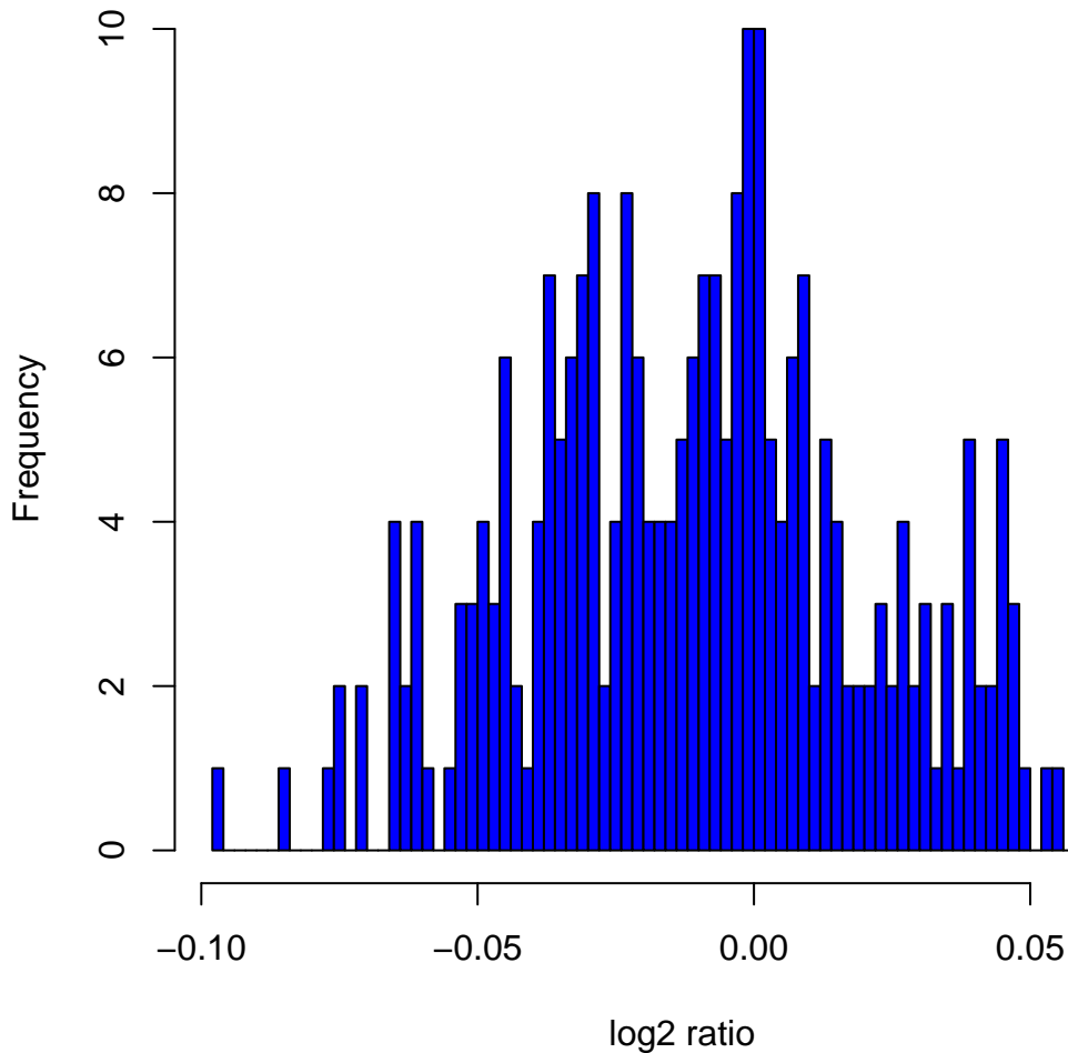
Histogram of log 2 ratios in 270 HapMap samples at clone Chr1tp-3H1
