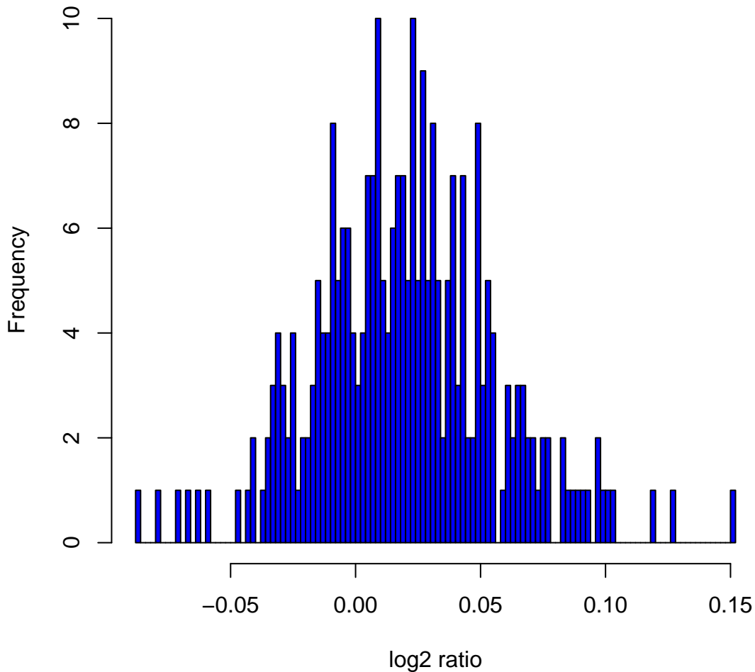
Histogram of log 2 ratios in 270 HapMap samples at clone Chr1tp-4A12
