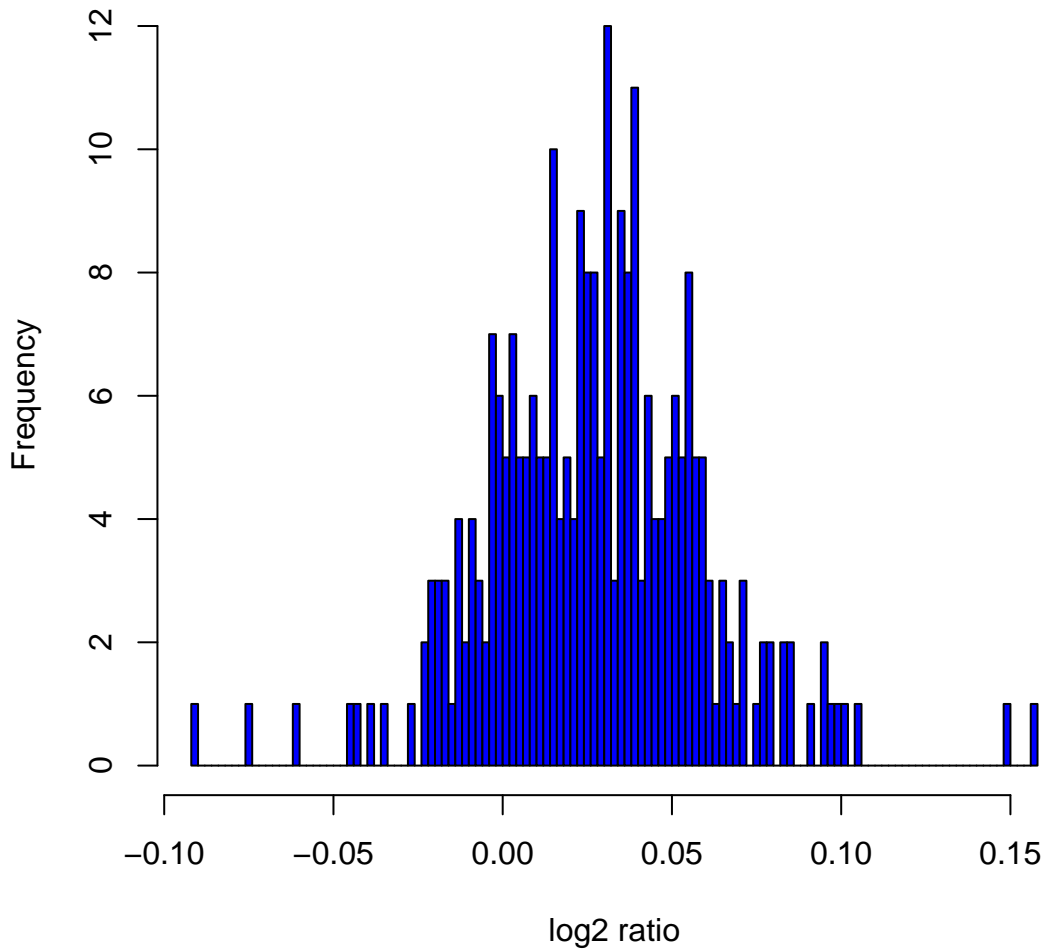
Histogram of log 2 ratios in 270 HapMap samples at clone Chr1tp-4D2
