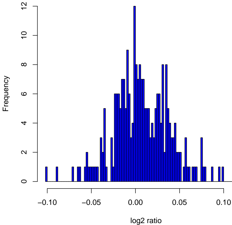
Histogram of log2ratios in 270 HapMap samples at clone Chr1tp-4F1
