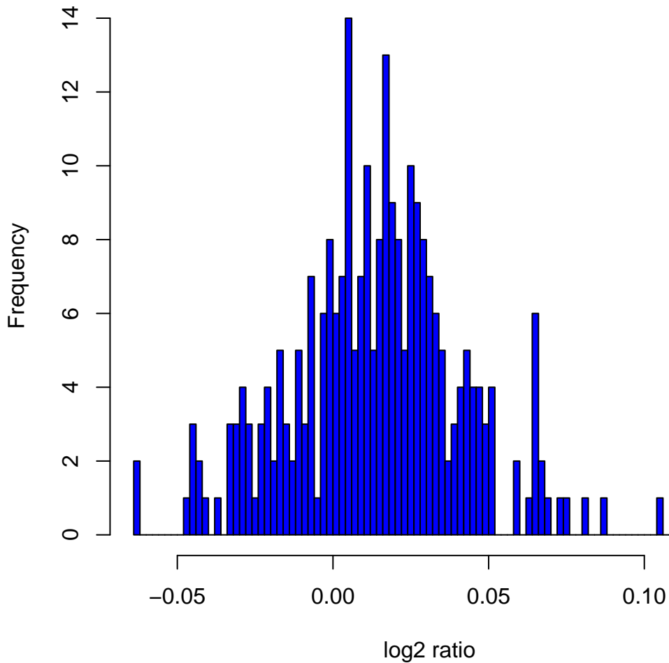
Histogram of log2ratios in 270 HapMap samples at clone Chr1tp-4H6
