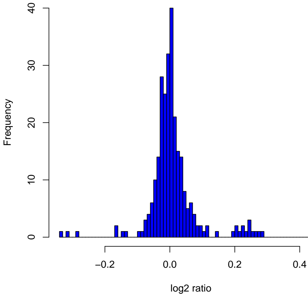
Histogram of \log_2 ratios in 270 HapMap samples at clone Chr1tp-5B3
