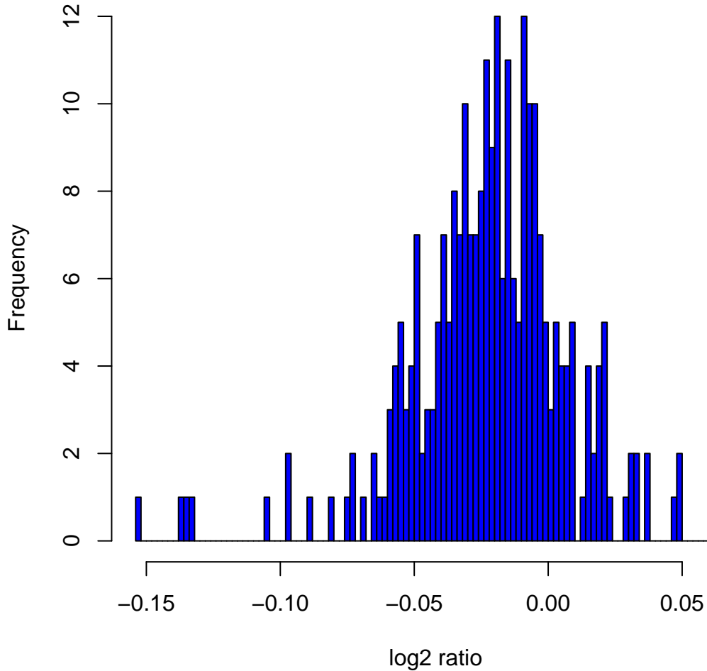
Histogram of log2ratios in 270 HapMap samples at clone Chr1tp-5F3
