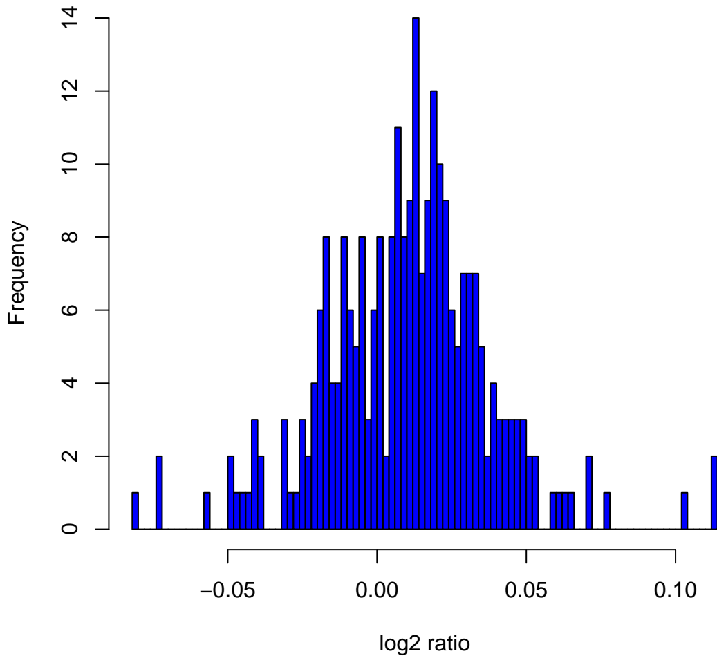
Histogram of log2ratios in 270 HapMap samples at clone Chr1tp-5G1
