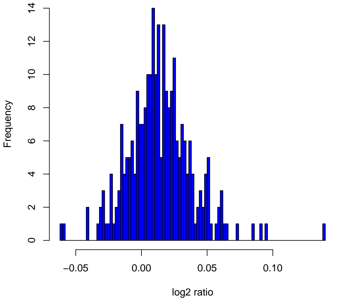
Histogram of \log_2 ratios in 270 HapMap samples at clone Chr1tp-5G2
