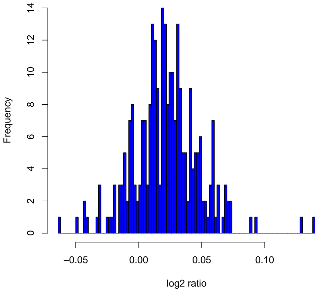
Histogram of \log_2 ratios in 270 HapMap samples at clone Chr1tp-5G3
