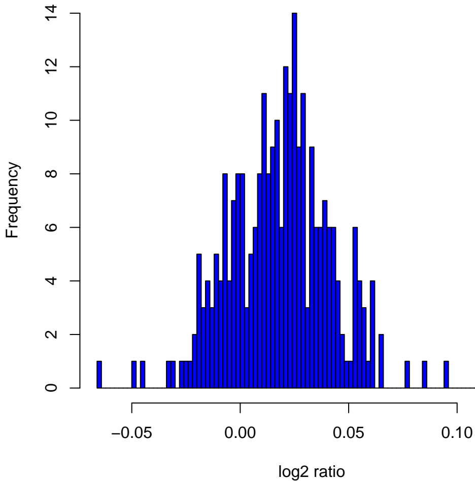
Histogram of log 2 ratios in 270 HapMap samples at clone Chr1tp-5G8
