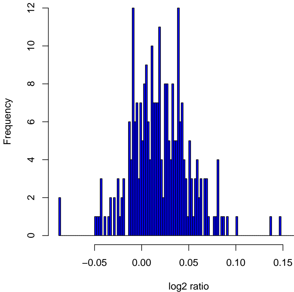
Histogram of log 2 ratios in 270 HapMap samples at clone Chr1tp-6A4
