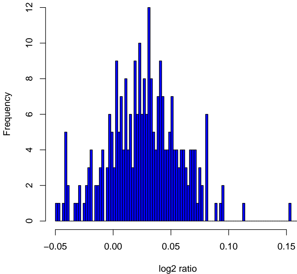
Histogram of \log_2 ratios in 270 HapMap samples at clone Chr1tp-6B6
