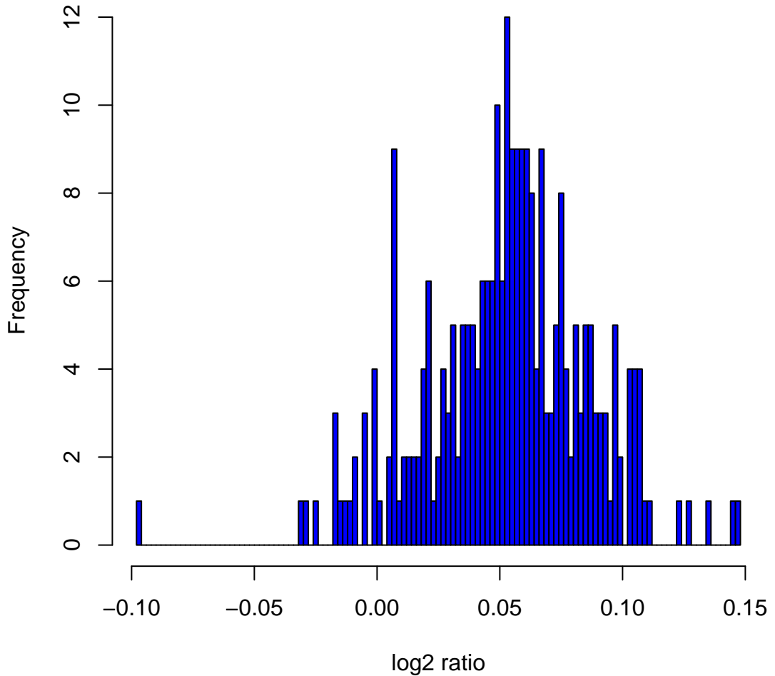
Histogram of log 2 ratios in 270 HapMap samples at clone Chr1tp-6C12
