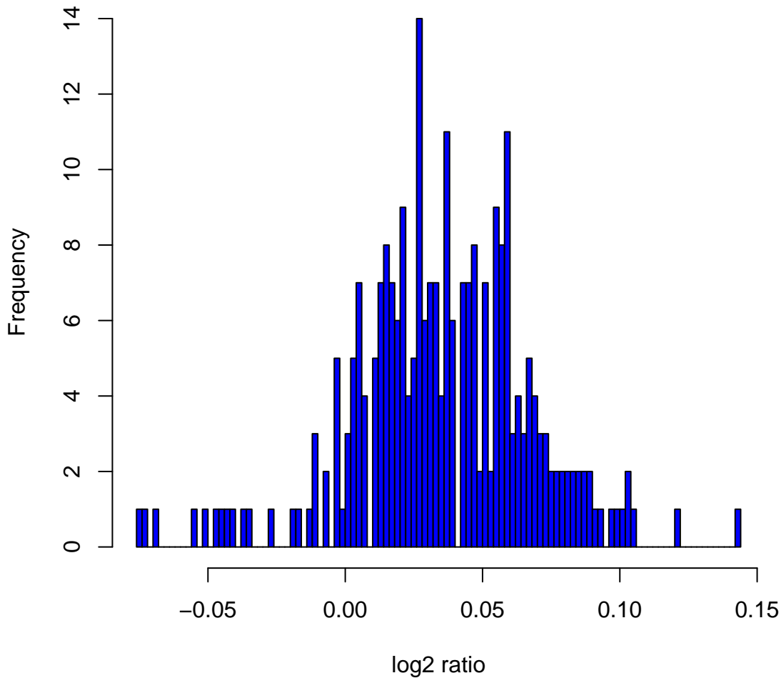
Histogram of log2ratios in 270 HapMap samples at clone Chr1tp-6E5
