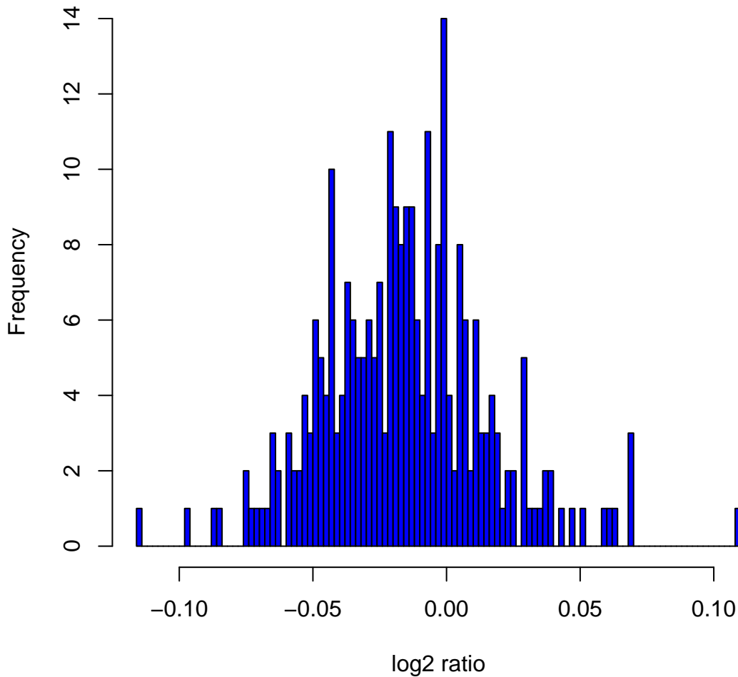
Histogram of log 2 ratios in 270 HapMap samples at clone Chr1tp-6G2
