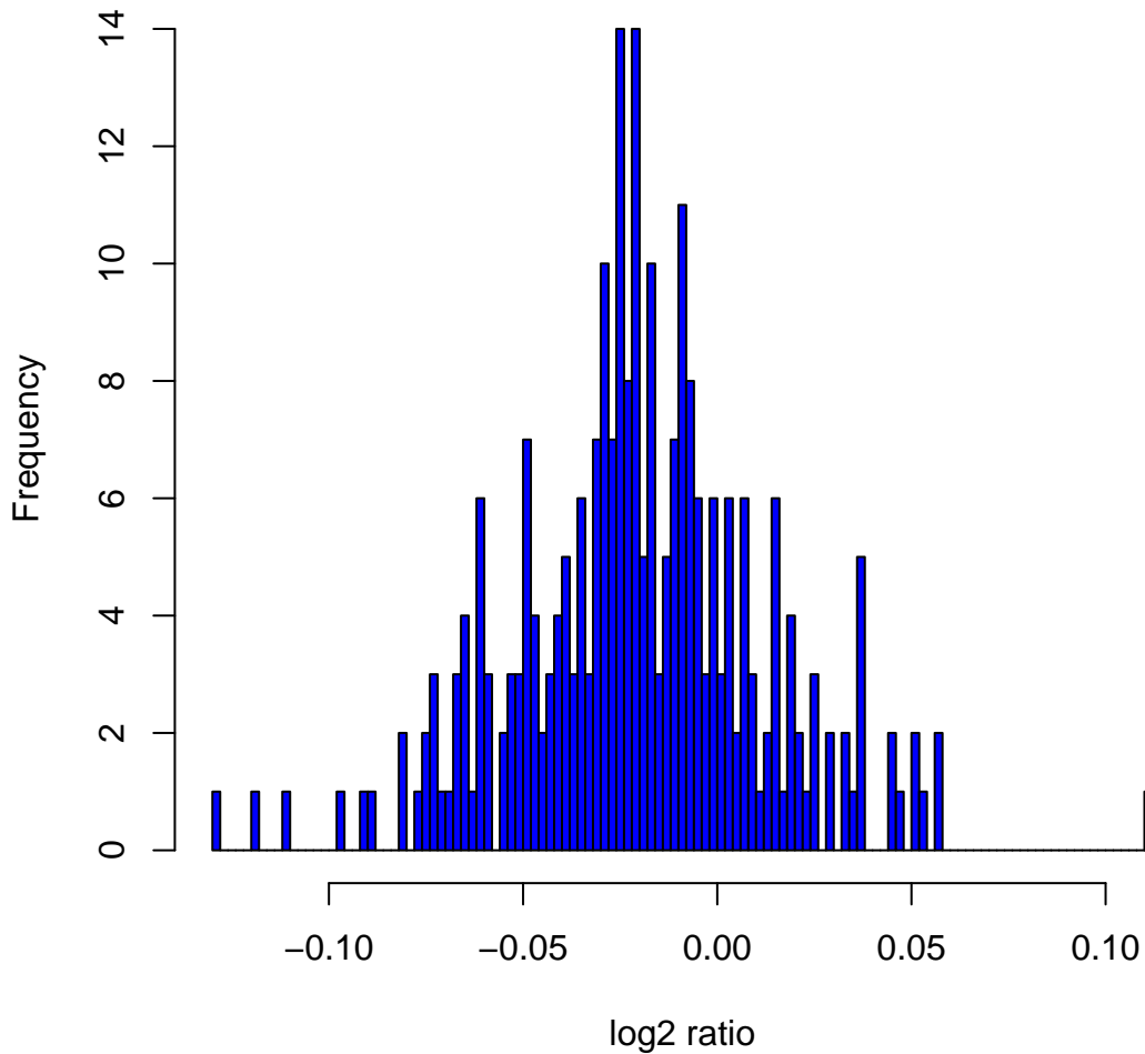
Histogram of log2ratios in 270 HapMap samples at clone Chr1tp-6H4
