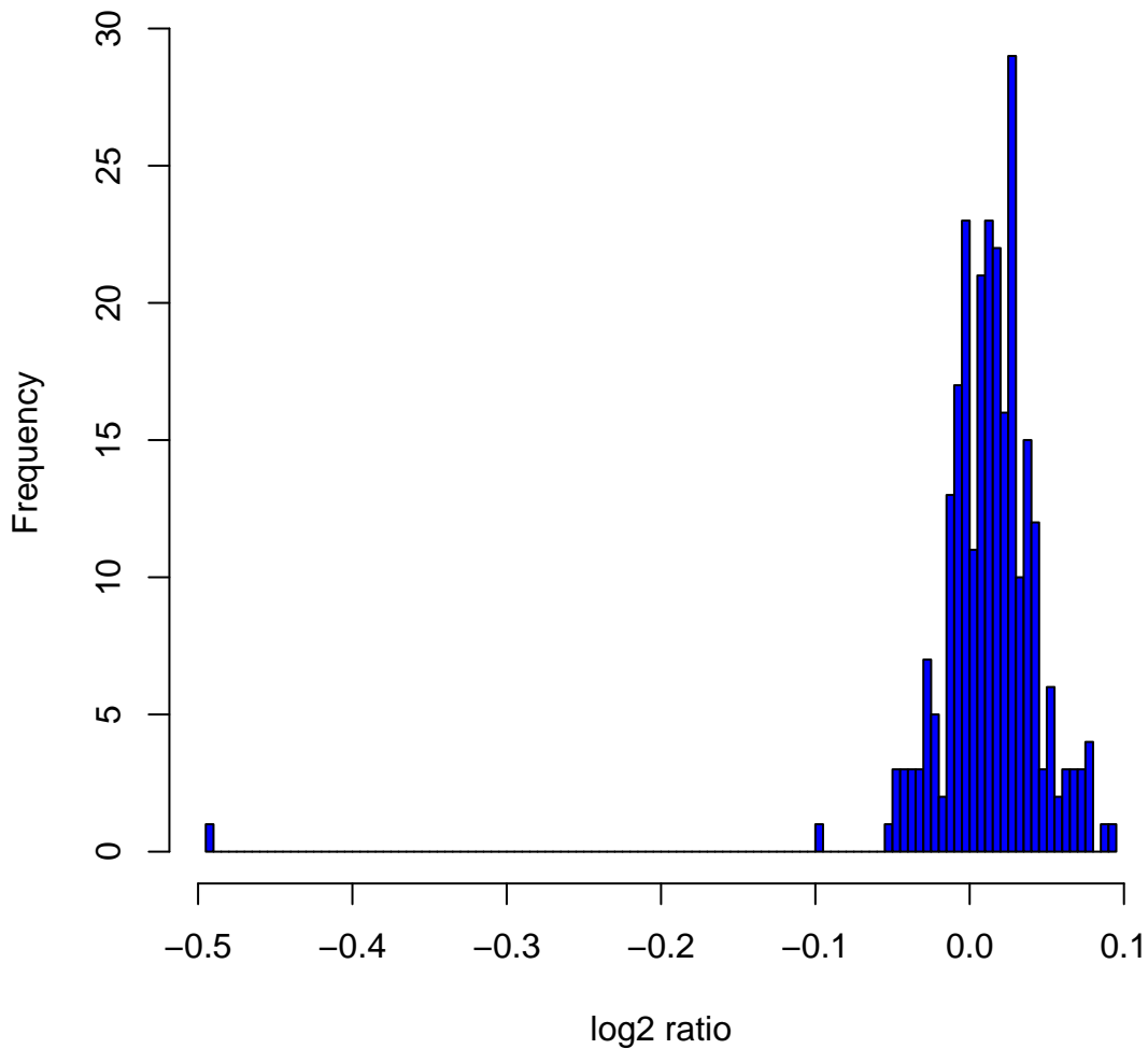
Histogram of log 2 ratios in 270 HapMap samples at clone Chr1tp-7B4
