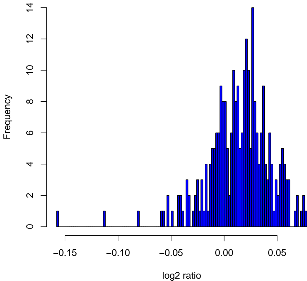
Histogram of log 2 ratios in 270 HapMap samples at clone Chr1tp-7C4
