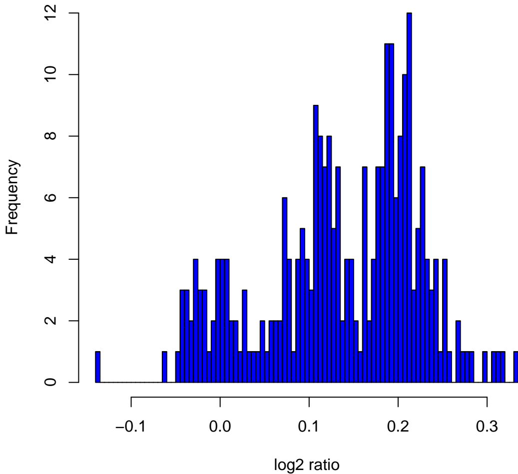
Histogram of \log_2 ratios in 270 HapMap samples at clone Chr1tp-7C8
