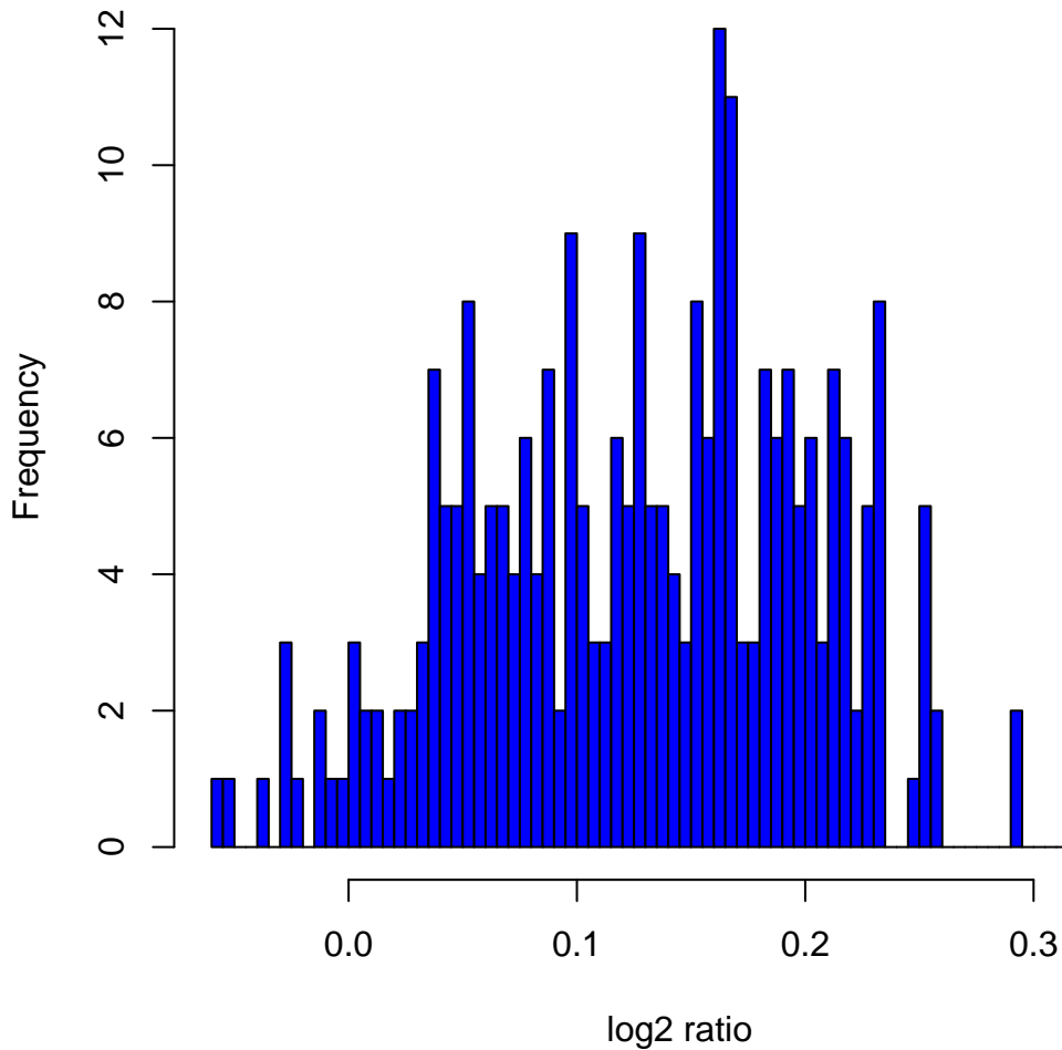
Histogram of log 2 ratios in 270 HapMap samples at clone Chr1tp-7D4
