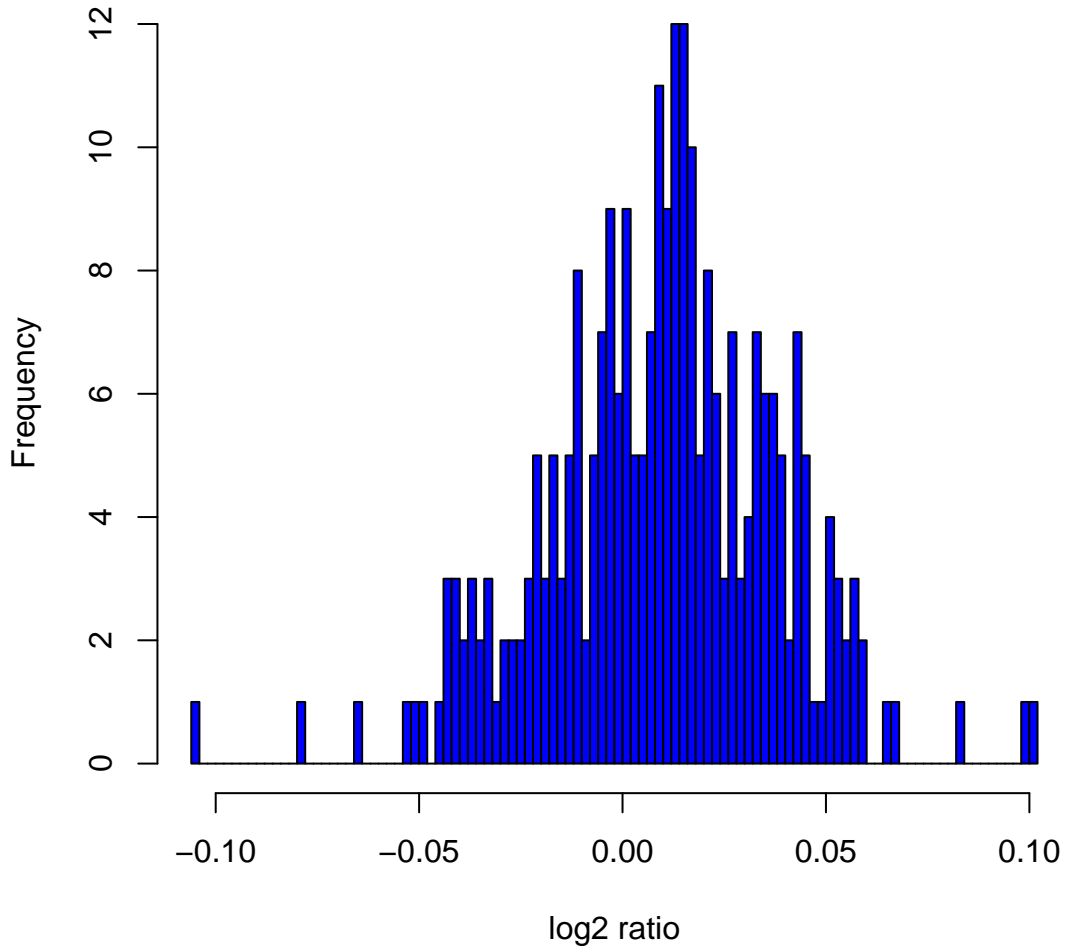
Histogram of log 2 ratios in 270 HapMap samples at clone Chr1tp-7E5
