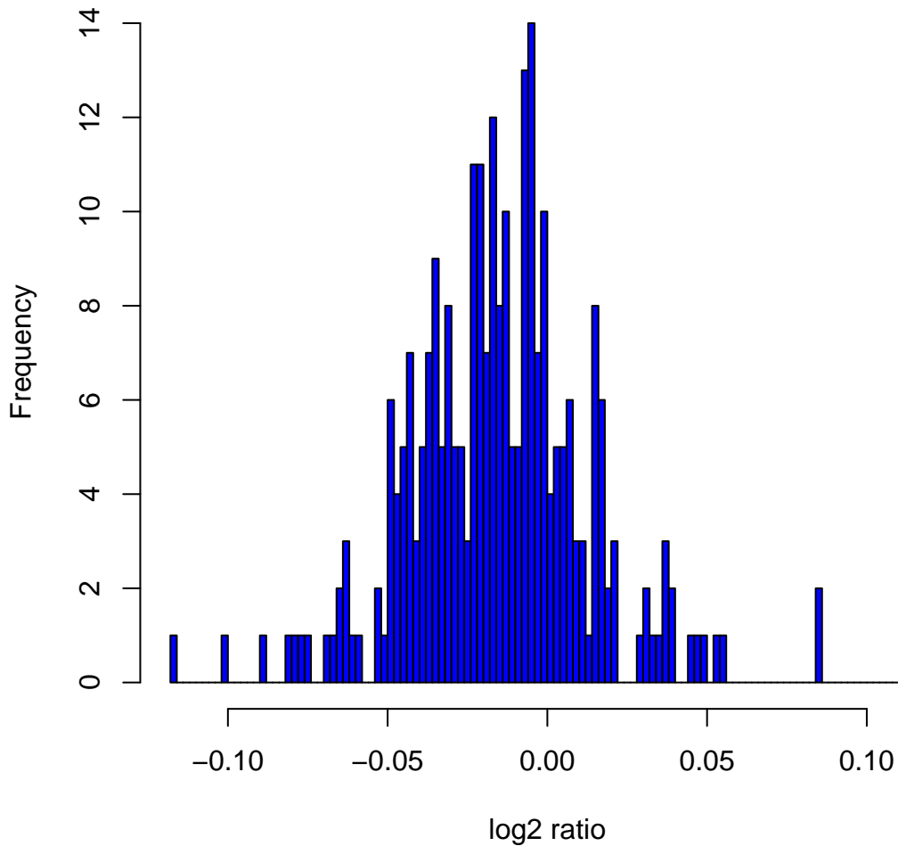
Histogram of log 2 ratios in 270 HapMap samples at clone Chr1tp-7E8
