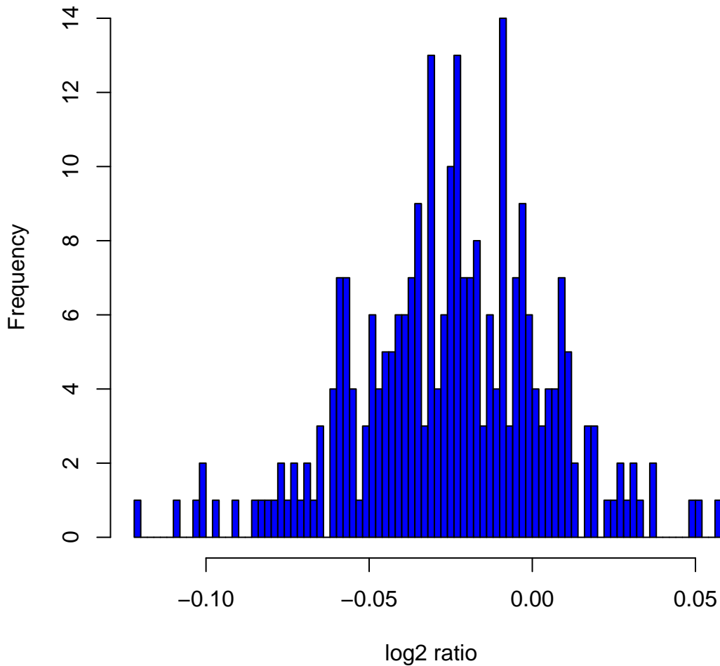
Histogram of \log_2 ratios in 270 HapMap samples at clone Chr1tp-8A5
