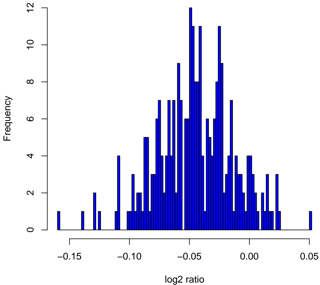
Histogram of \log_2 ratios in 270 HapMap samples at clone Chr1tp-8A9
