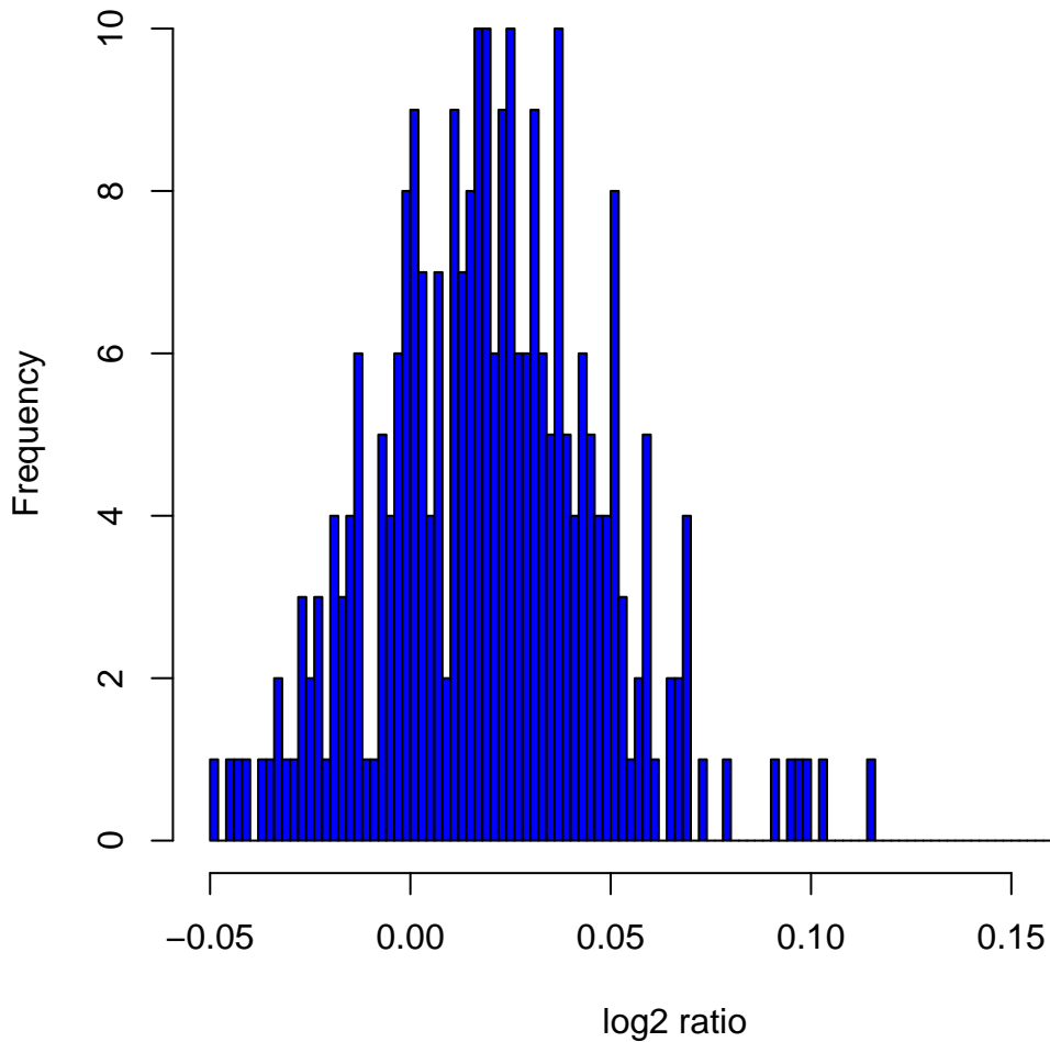
Histogram of log 2 ratios in 270 HapMap samples at clone Chr1tp-8C1
