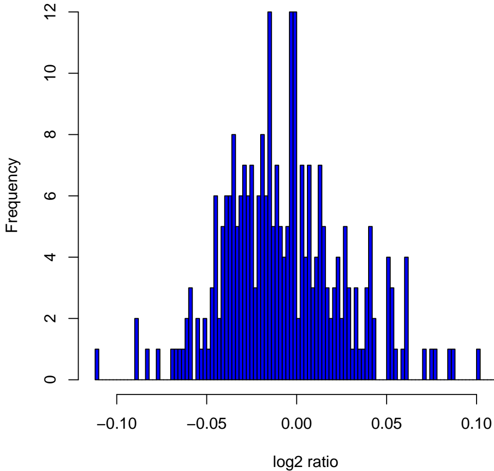
Histogram of \log_2 ratios in 270 HapMap samples at clone Chr1tp-8C11
