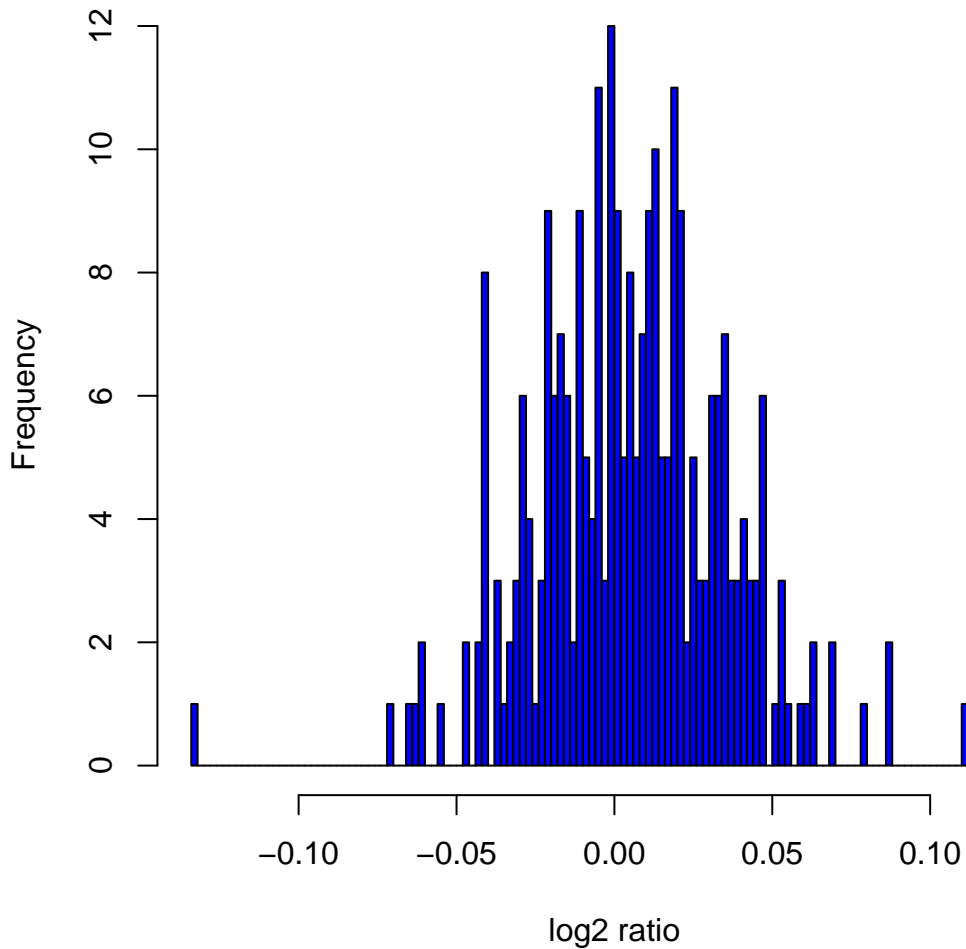
Histogram of \log_2 ratios in 270 HapMap samples at clone Chr1tp-8C3
