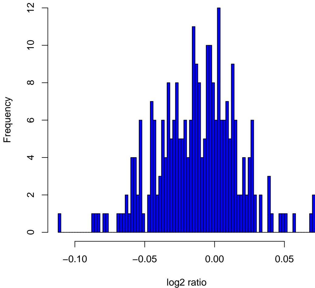
Histogram of \log_2 ratios in 270 HapMap samples at clone Chr1tp-8C9
