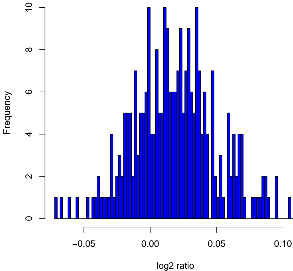
Histogram of log 2 ratios in 270 HapMap samples at clone Chr1tp-8F10
