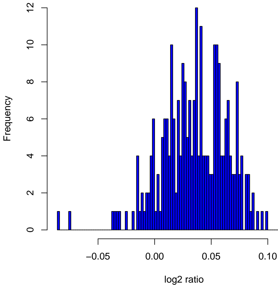
Histogram of log2ratios in 270 HapMap samples at clone Chr1tp-8F2
