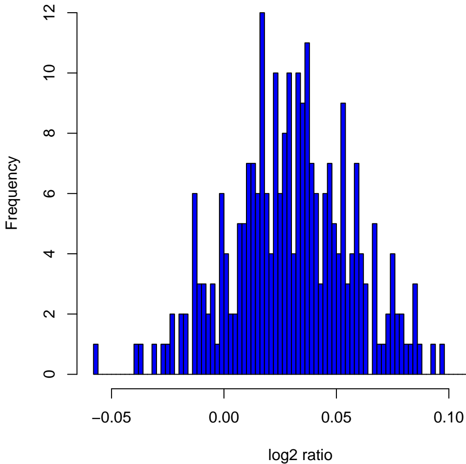
Histogram of \log_2 ratios in 270 HapMap samples at clone Chr1tp-9B5
