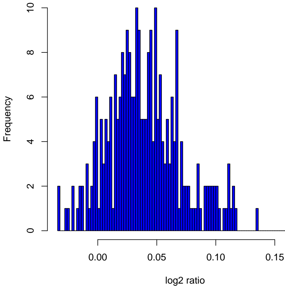
Histogram of \log_2 ratios in 270 HapMap samples at clone Chr1tp-9C10
