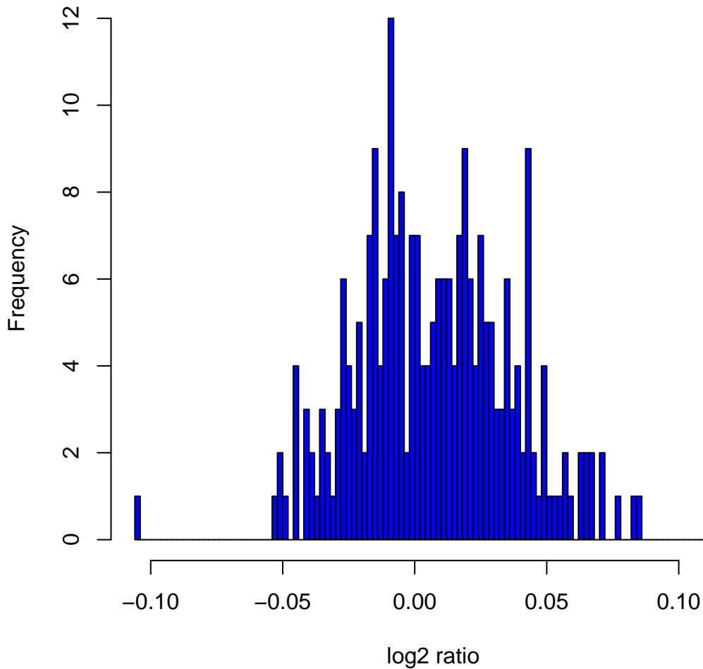
Histogram of \log_2 ratios in 270 HapMap samples at clone Chr1tp-9C3
