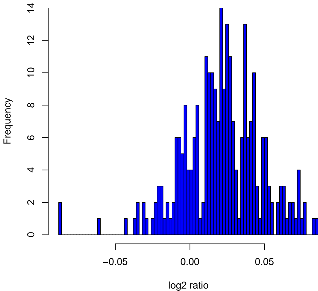
Histogram of log 2 ratios in 270 HapMap samples at clone Chr1tp-9G12
