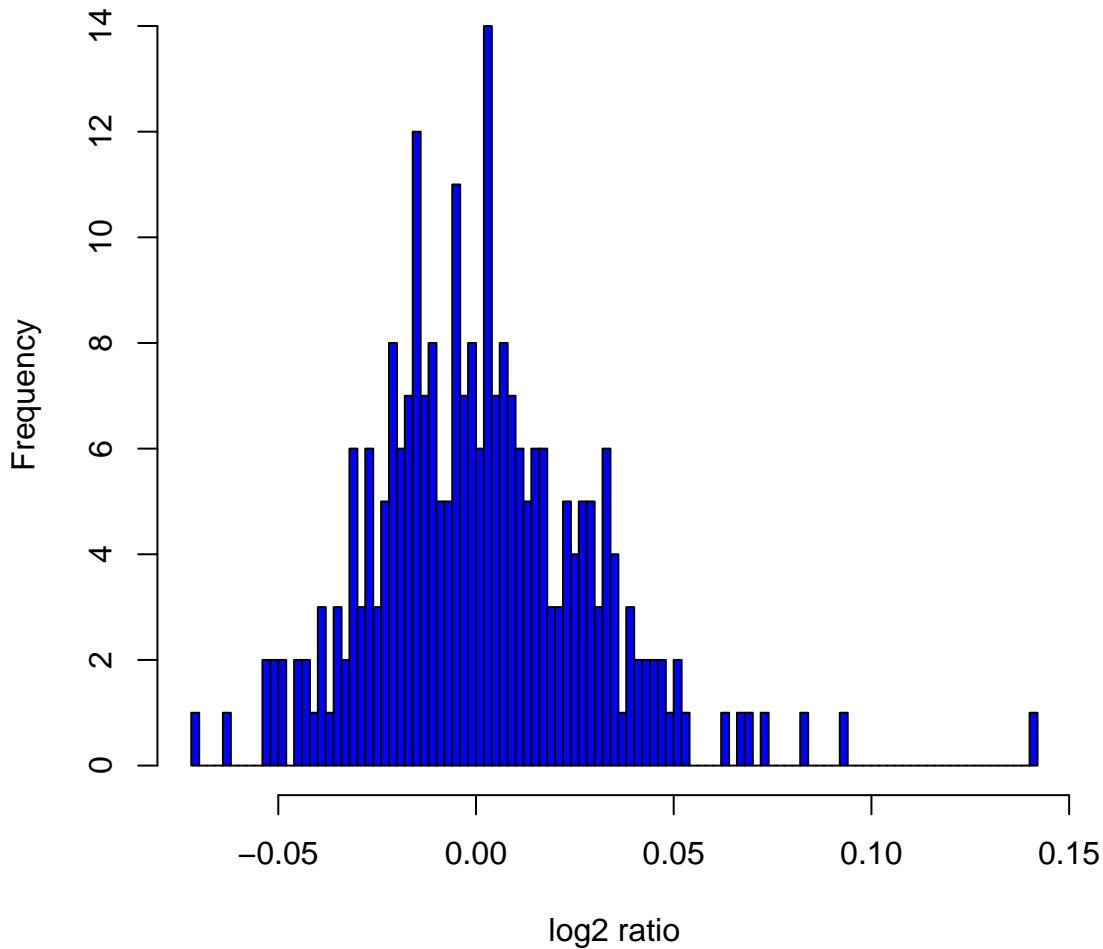
Histogram of log 2 ratios in 270 HapMap samples at clone Chr1tp-9G3
