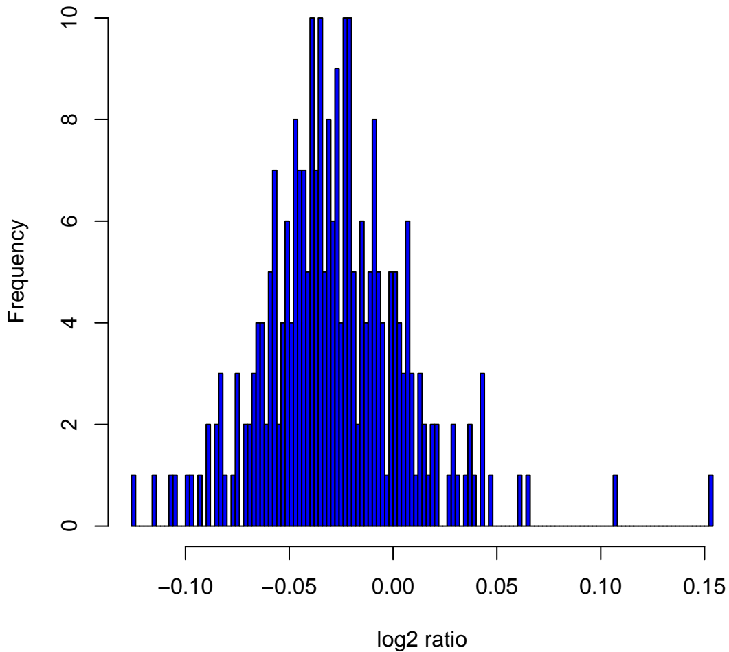
Histogram of \log_2 ratios in 270 HapMap samples at clone Chr6tp-19C8
