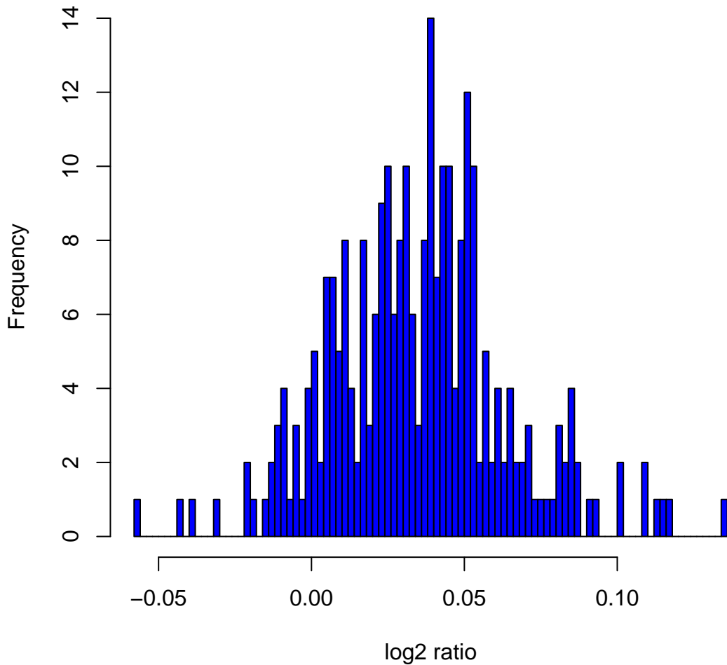
Histogram of \log_2 ratios in 270 HapMap samples at clone Chr10tp-10B11
