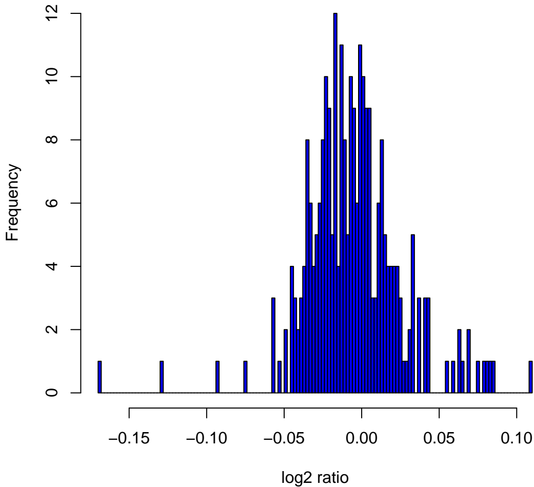
Histogram of log2ratios in 270 HapMap samples at clone Chr10tp-10C7
