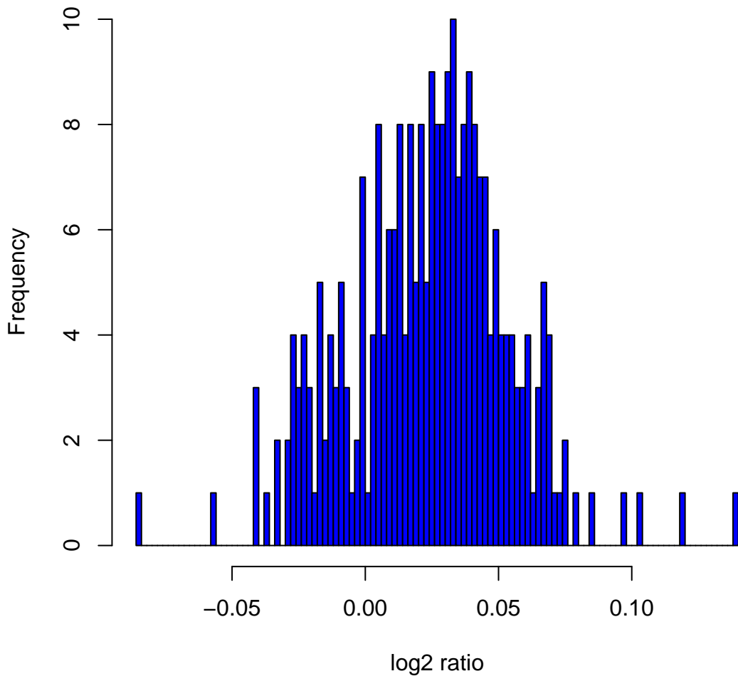
Histogram of log2ratios in 270 HapMap samples at clone Chr10tp-10D11
