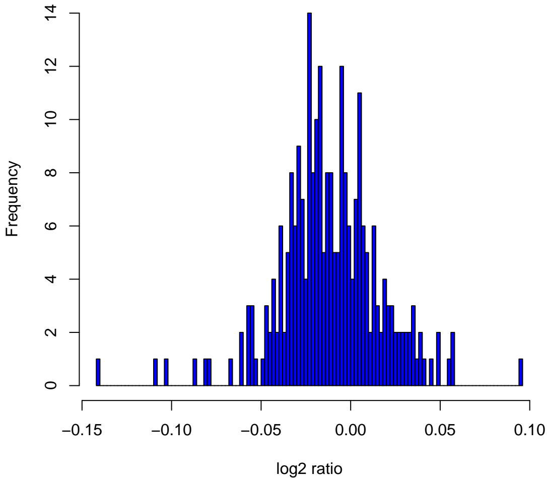
Histogram of log2ratios in 270 HapMap samples at clone Chr10tp-10D8
