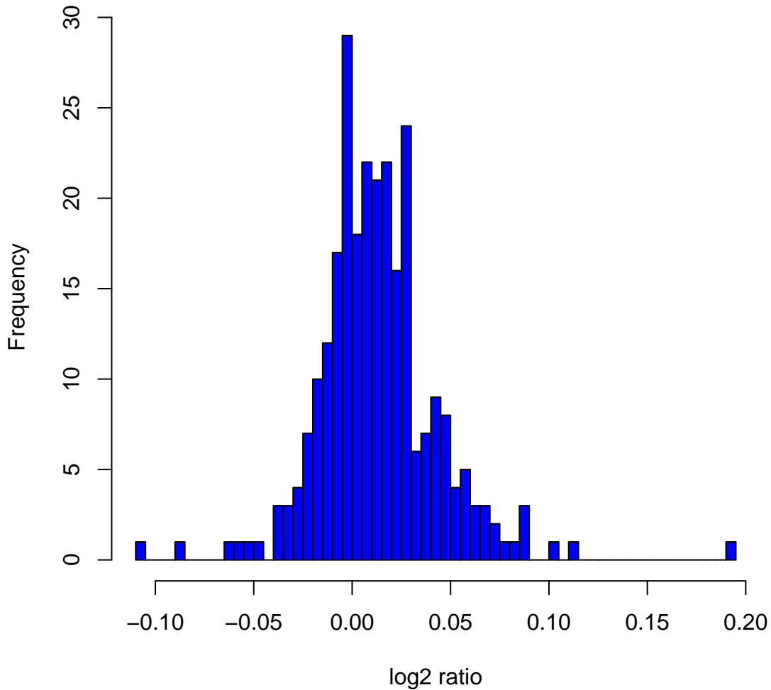
Histogram of log2ratios in 270 HapMap samples at clone Chr10tp-10F6
