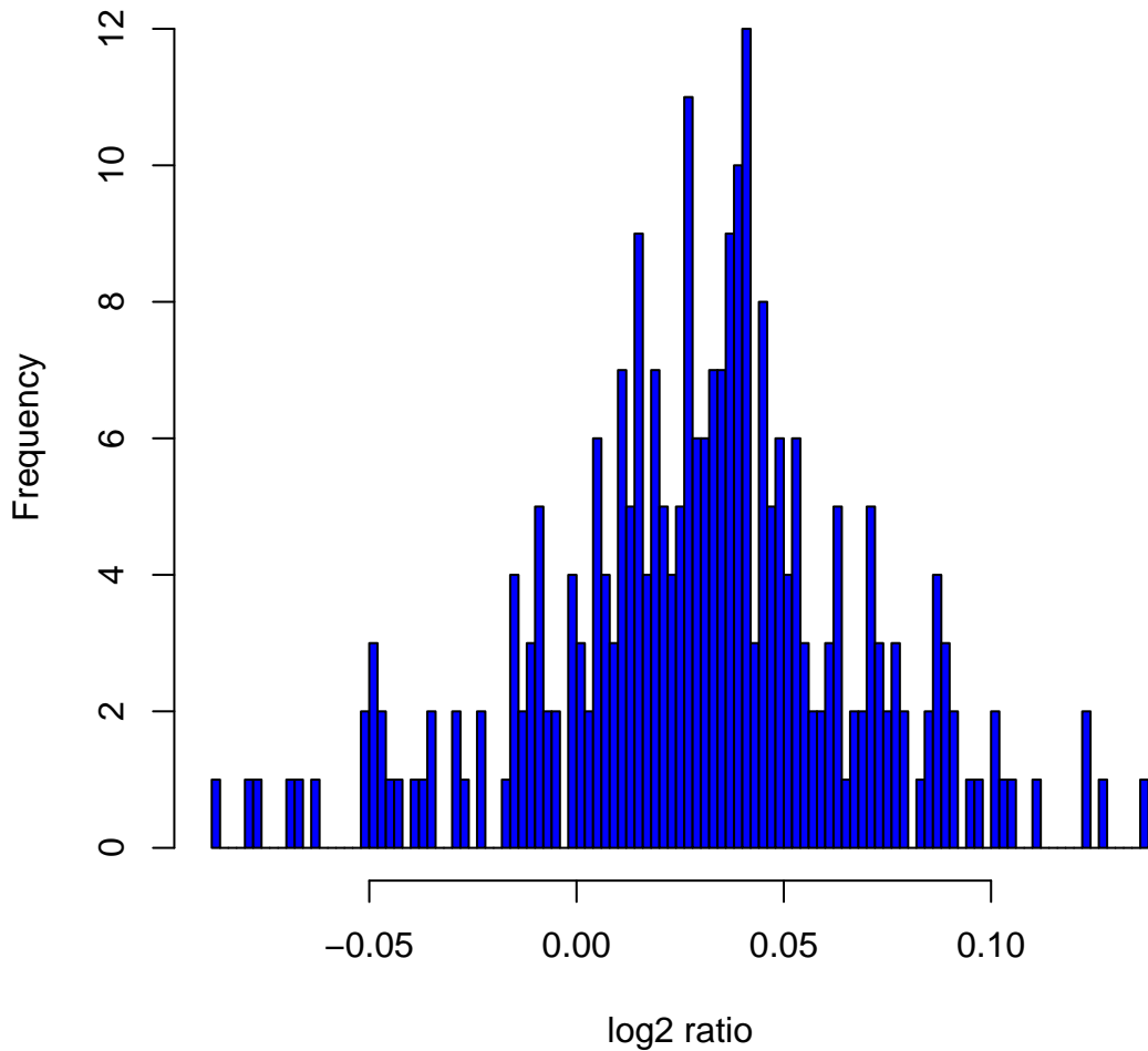
Histogram of log2ratios in 270 HapMap samples at clone Chr10tp-11B4
