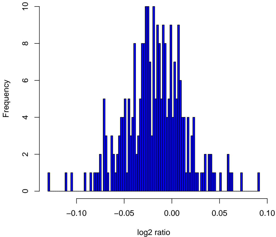
Histogram of log2ratios in 270 HapMap samples at clone Chr10tp-11D7
