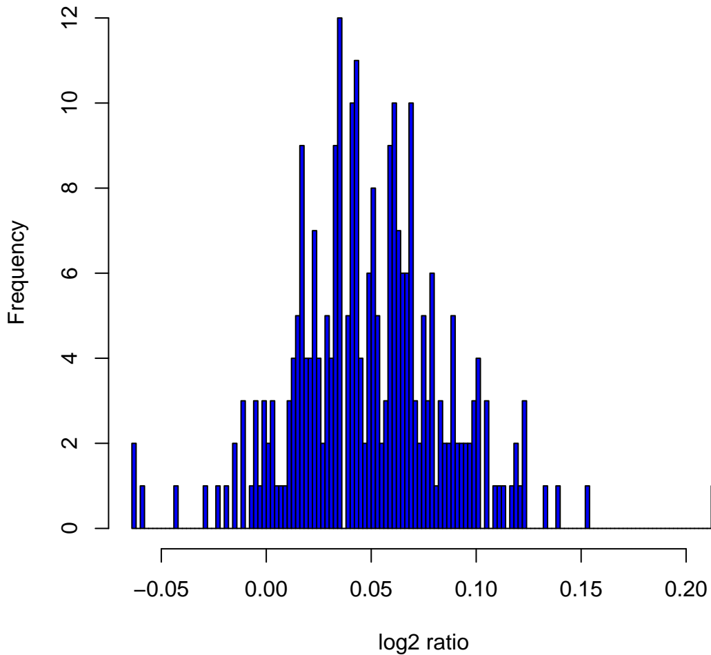
Histogram of log2ratios in 270 HapMap samples at clone Chr10tp-11H4
