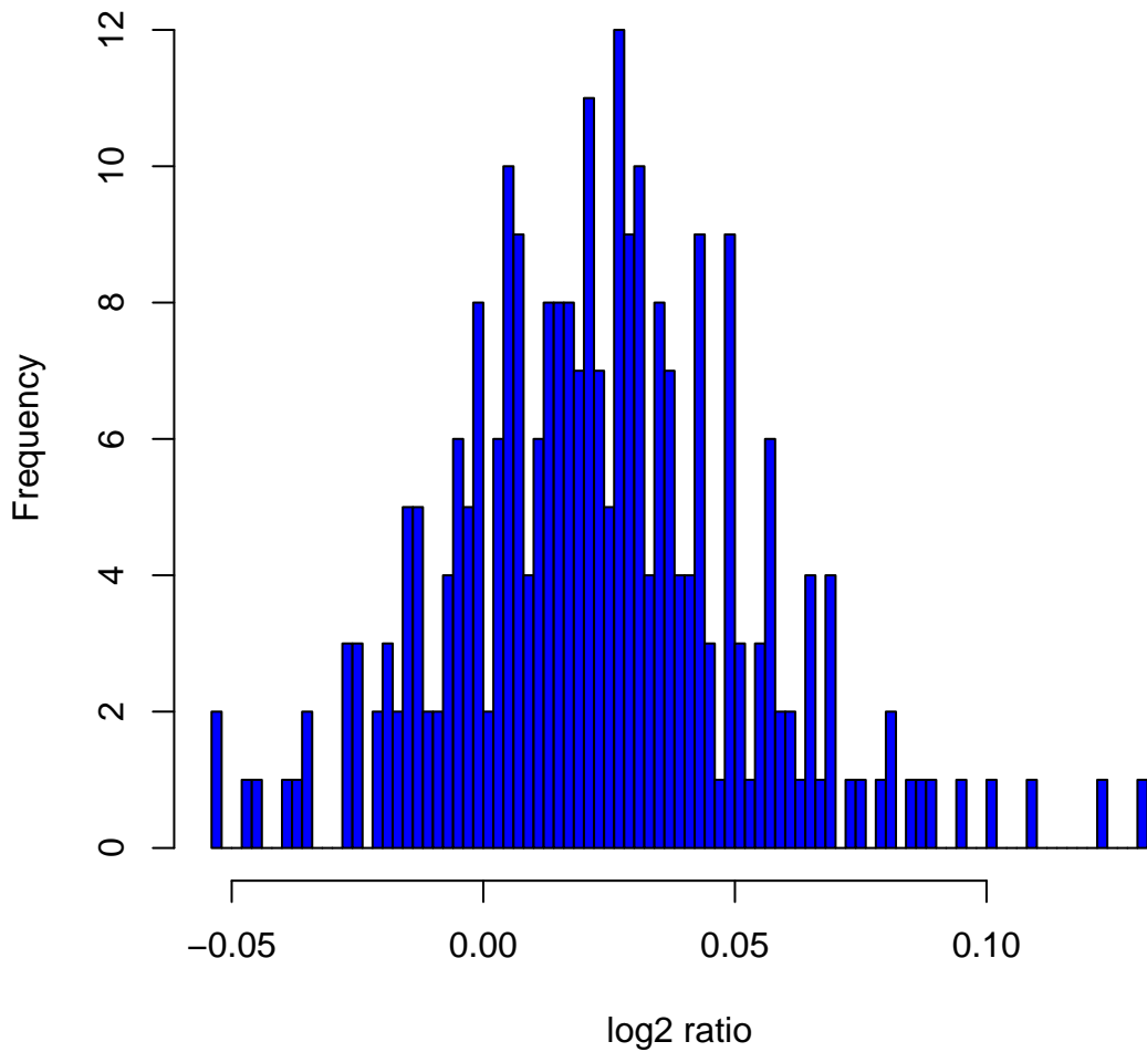
Histogram of log2ratios in 270 HapMap samples at clone Chr10tp-12A12
