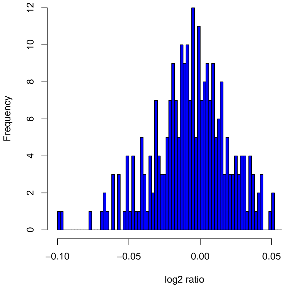
Histogram of log2ratios in 270 HapMap samples at clone Chr10tp-12B8
