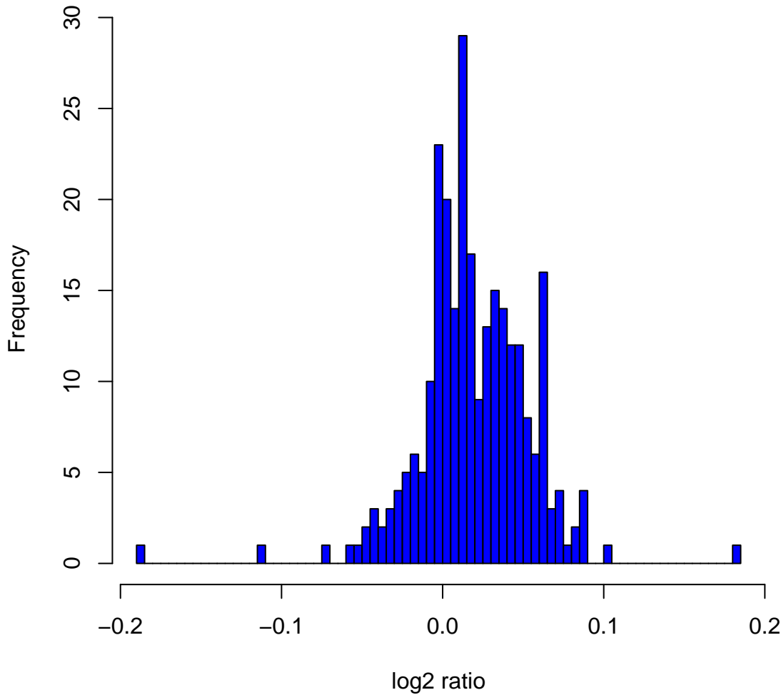
Histogram of log2ratios in 270 HapMap samples at clone Chr10tp-12D10
