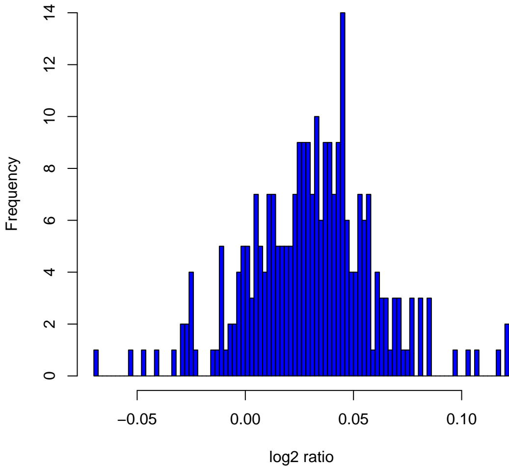
Histogram of log2ratios in 270 HapMap samples at clone Chr10tp-12D3
